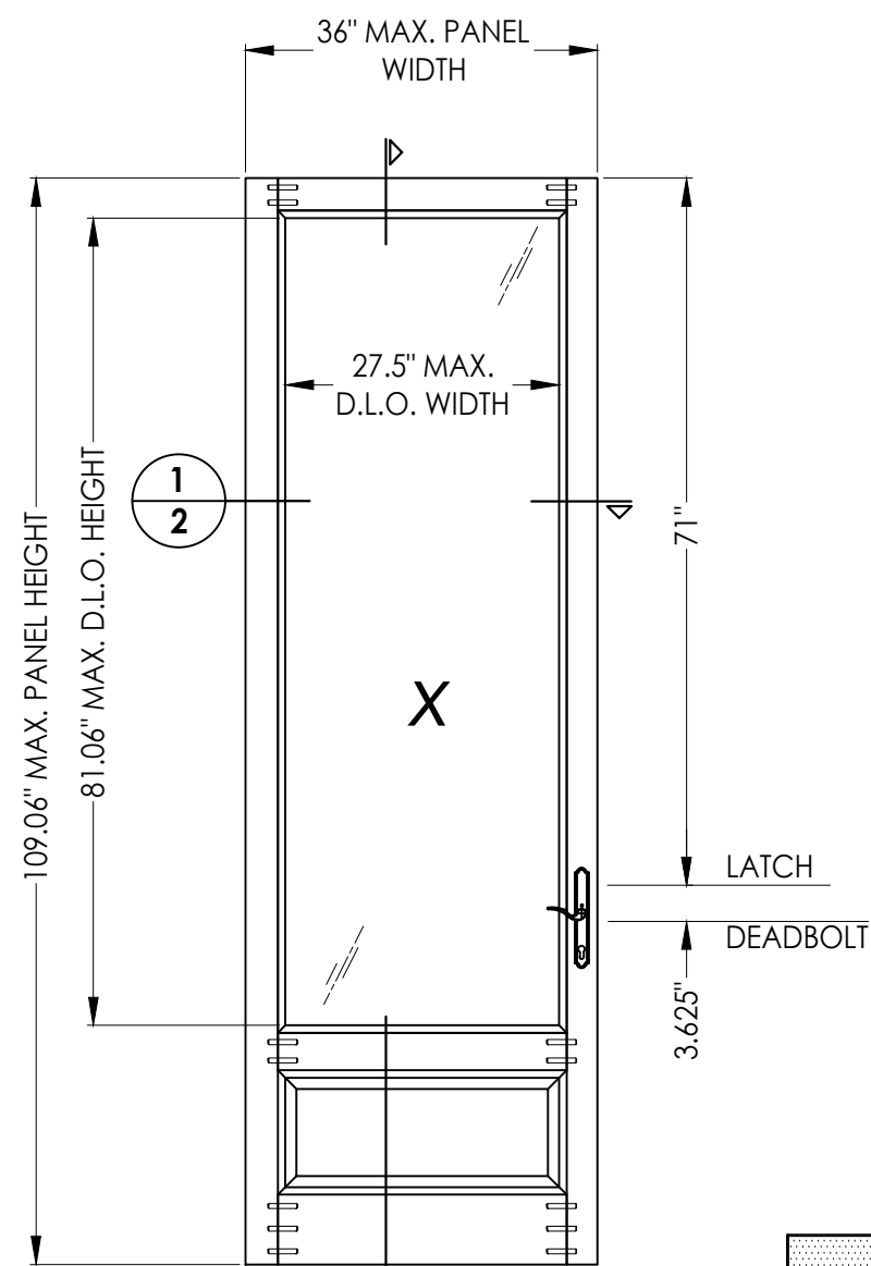
2 2 WOOD DOOR PANEL MW MILLWORKS
