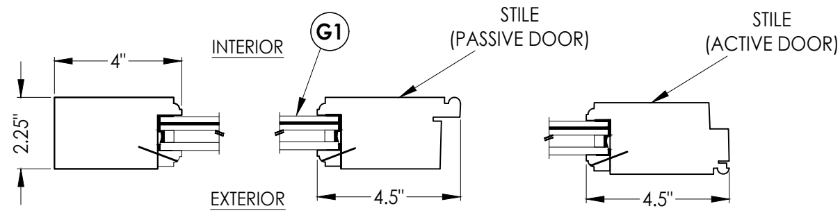
1 2 HORIZONTAL CROSS SECTION
